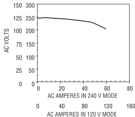
GENERATOR POWER CURVE
